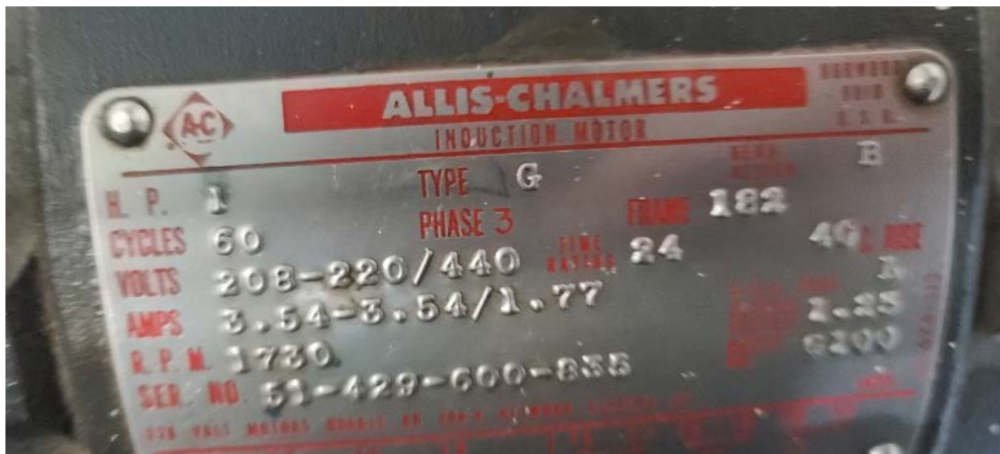
Vacuum Motor Name Plate
